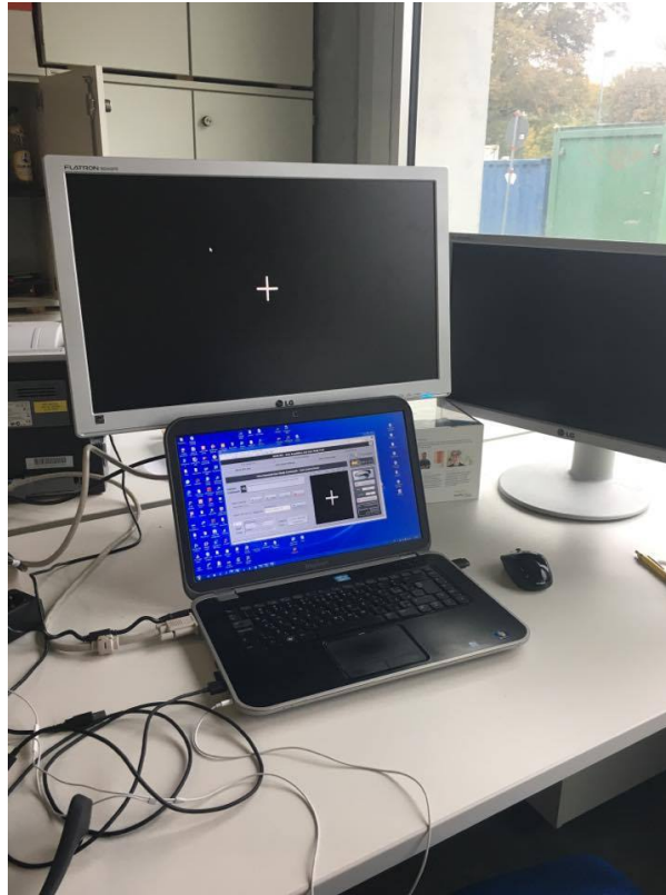
Figure 4.12: System Setup: Laptop is running the test and recording the videos and above is the black screen with the fixation cross
